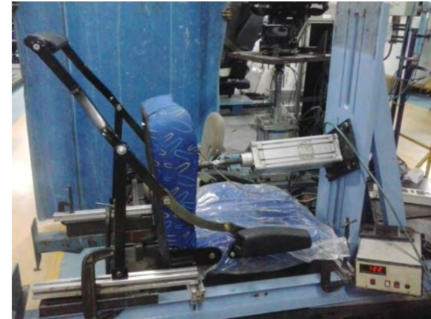
Vertical strength test for co- driver
